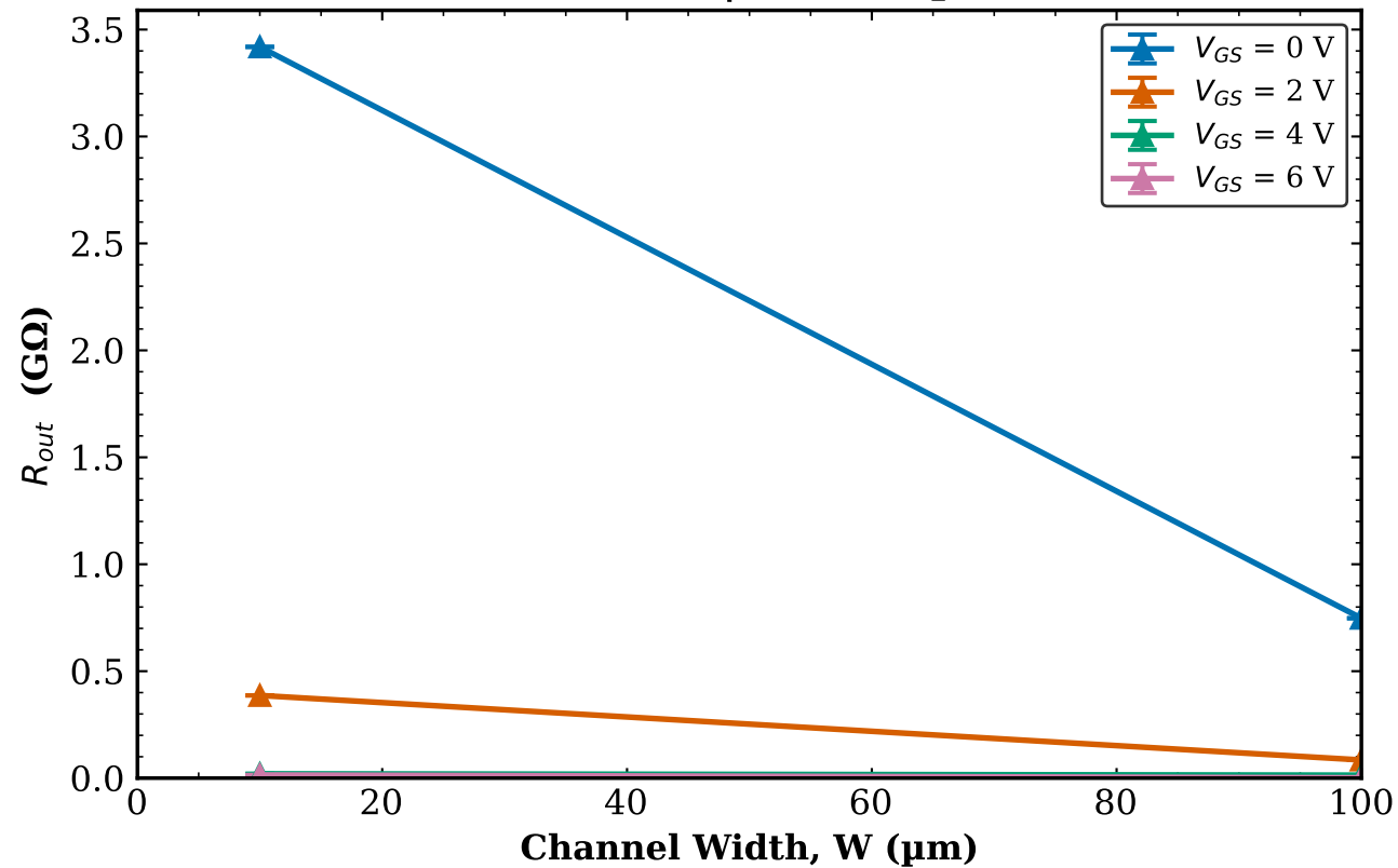
TFT2 Transistor 2 R_{out} vs W | L = 80\text{ }\mu\text{m}
